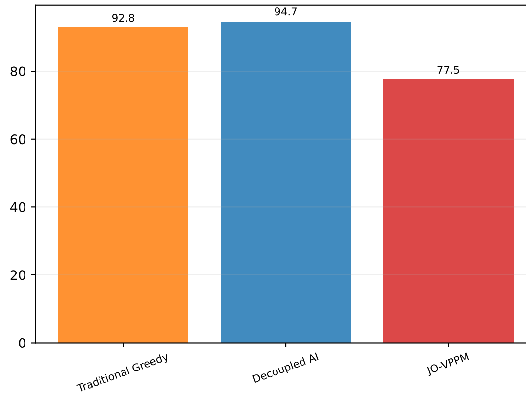
M/G/1 Queue Latency (ms)
