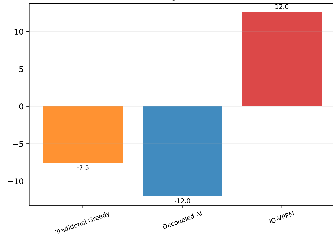
Average Reward
