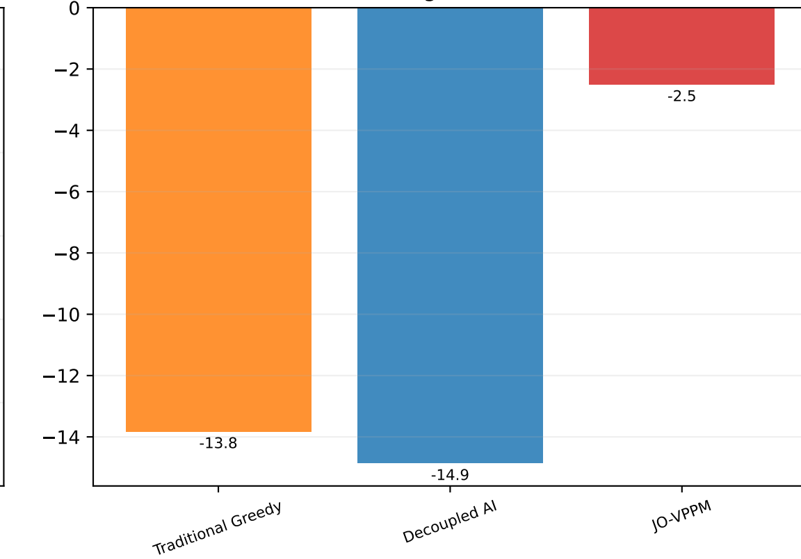
Average Reward
