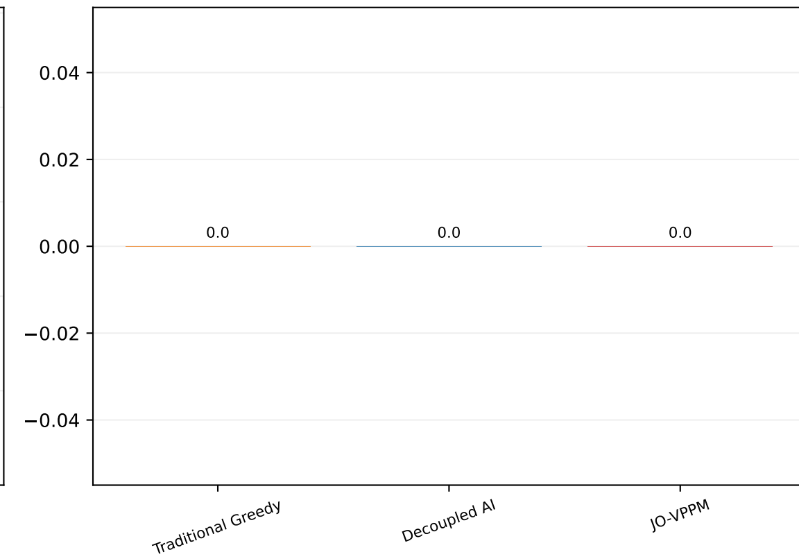
Average Reward
