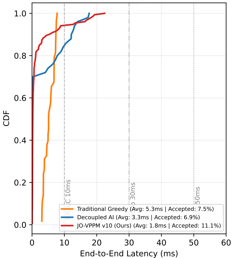
Latency CDF (Accepted Only) — NSFNET (Bursty)
