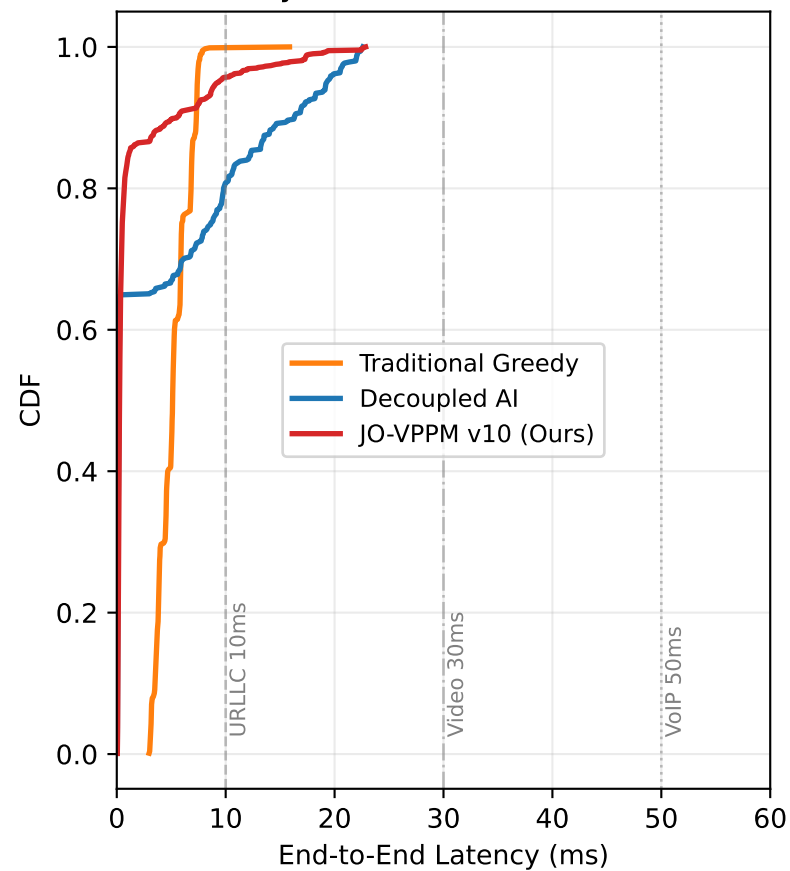
Latency CDF — NSFNET (Uniform)
