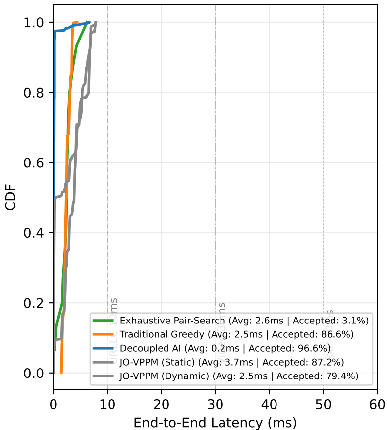
Latency CDF (Accepted Only) — VIETNAM (Bursty)
