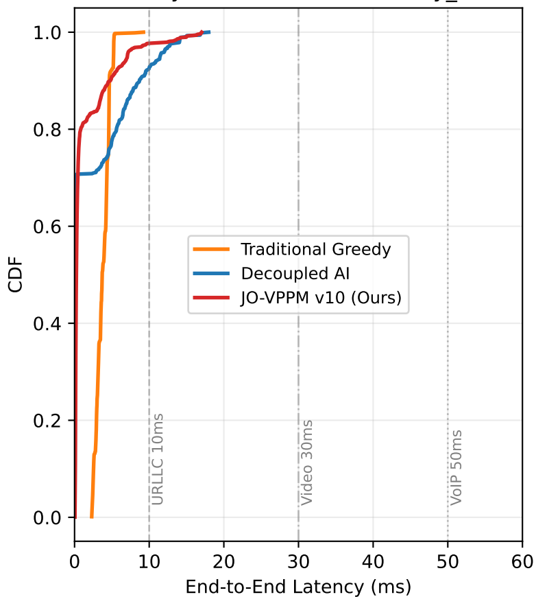
Latency CDF — GEANT2 (Heavy_tail)
