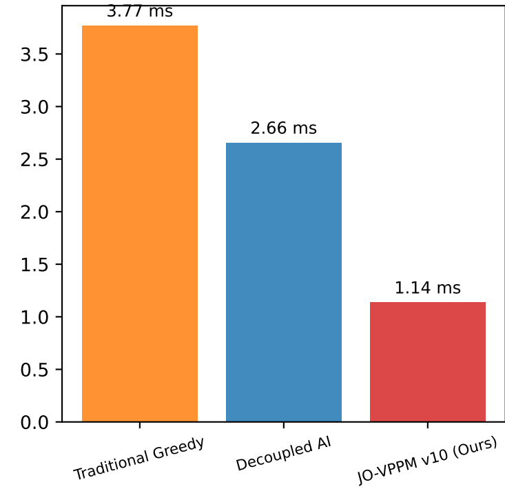
Average Latency (ms)
