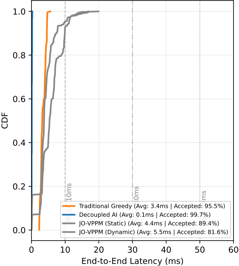
Latency CDF (Accepted Only) — GEANT2 (Uniform)
