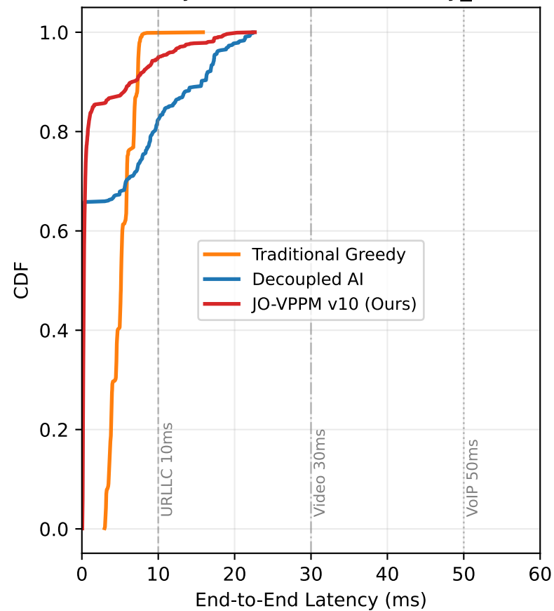
Latency CDF — NSFNET (Heavy_tail)
