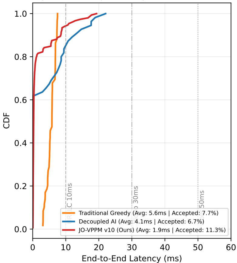
Latency CDF (Accepted Only) — NSFNET (Uniform)
