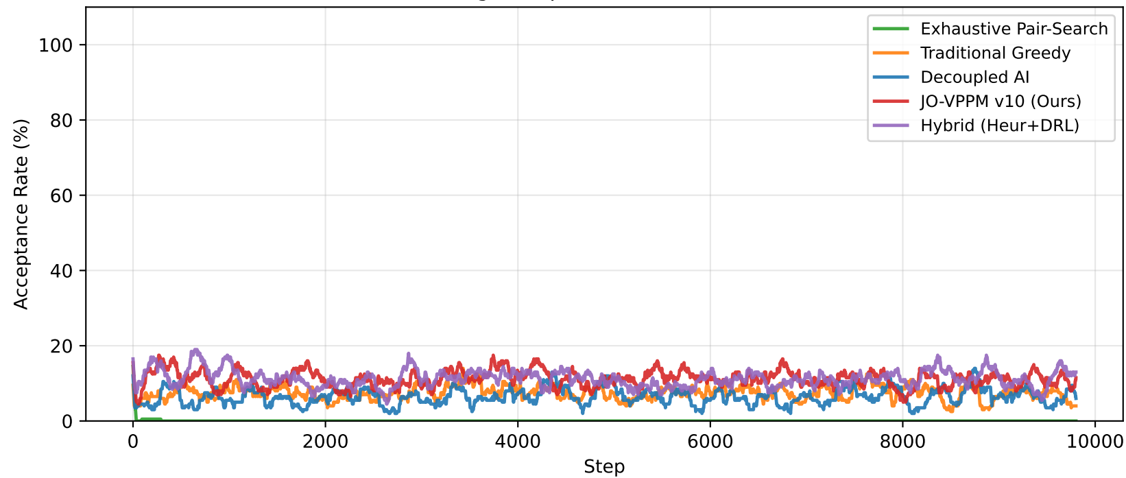
Rolling Acceptance (window=200)
