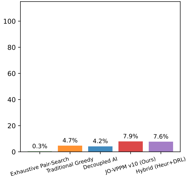
Acceptance Rate (%)
