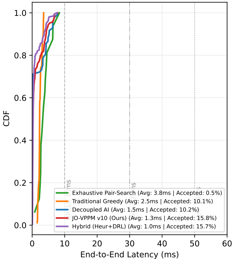
Latency CDF (Accepted Only) — VIETNAM (Spike)
