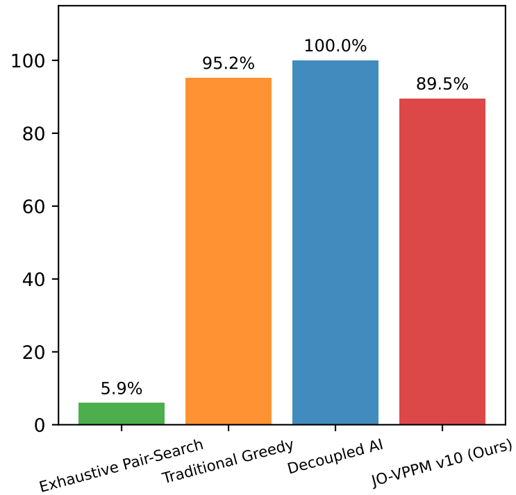
Acceptance Rate (%)
