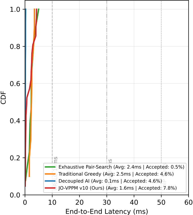
Latency CDF (Accepted Only) — VIETNAM (Uniform)
