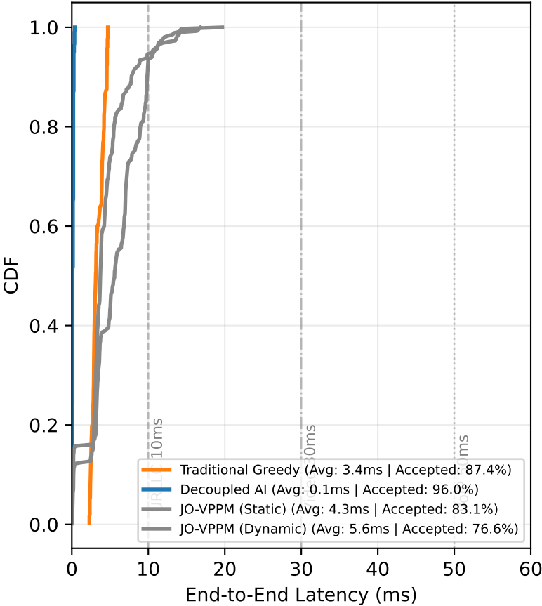
Latency CDF (Accepted Only) — GEANT2 (Heavy_tail)
