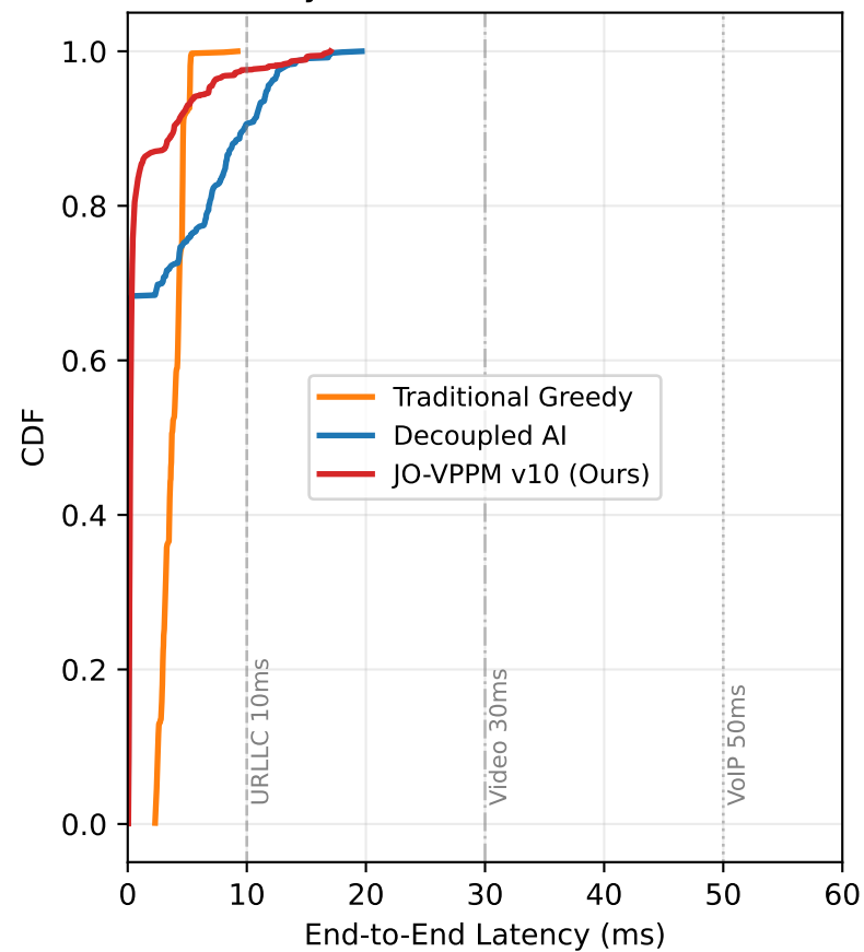
Latency CDF — GEANT2 (Uniform)
