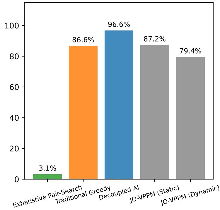
Acceptance Rate (%)
