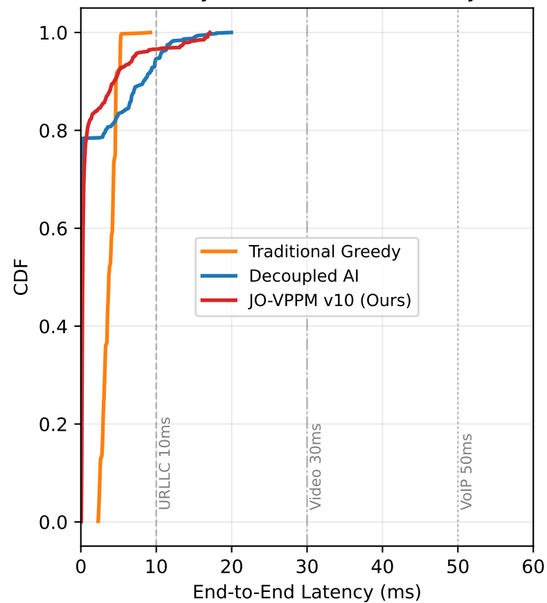
Latency CDF — GEANT2 (Bursty)
