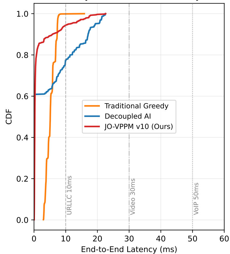
Latency CDF — NSFNET (Bursty)
