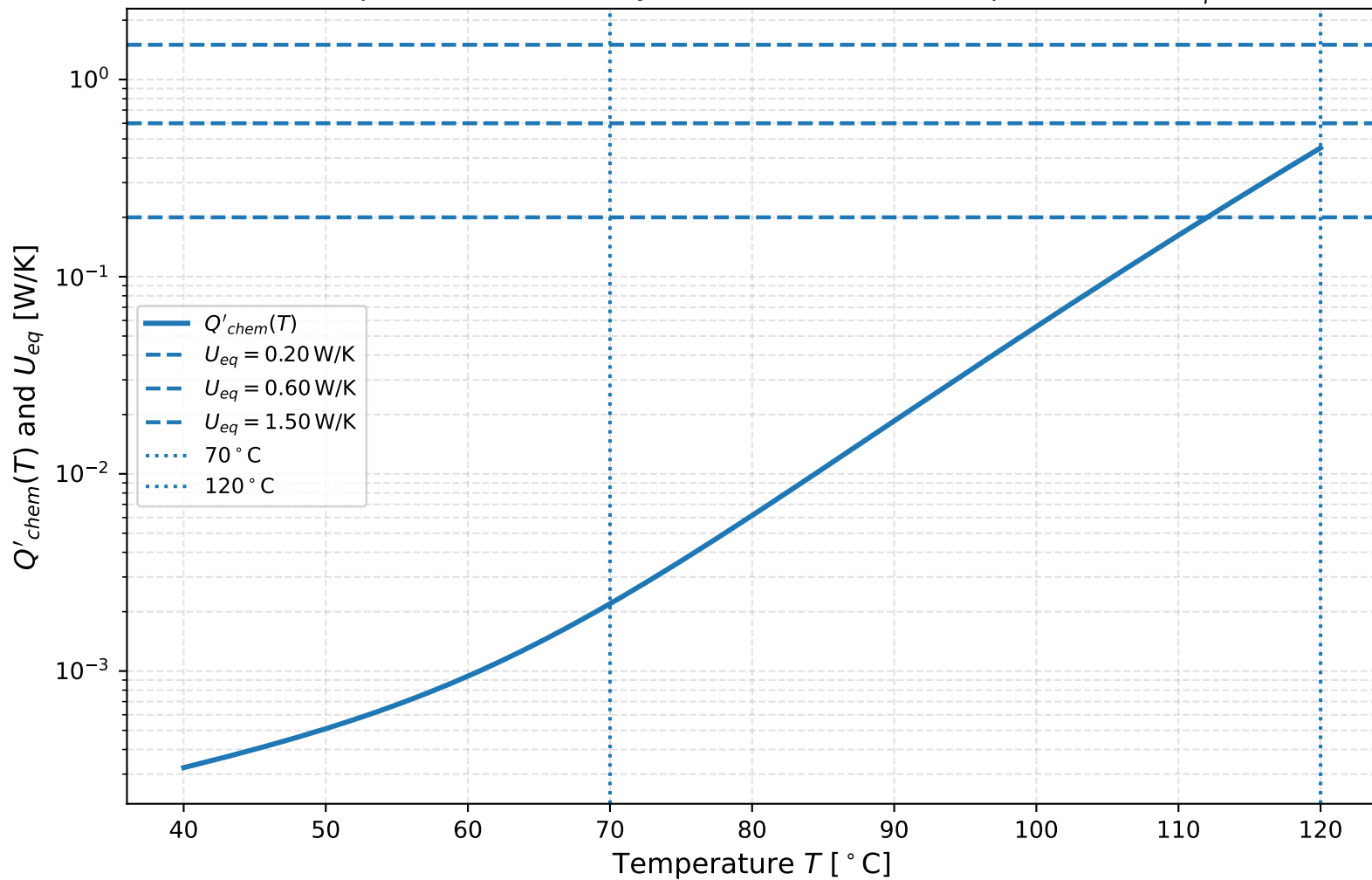
Temperature sensitivity of chemical heat compared with U_{eq}
