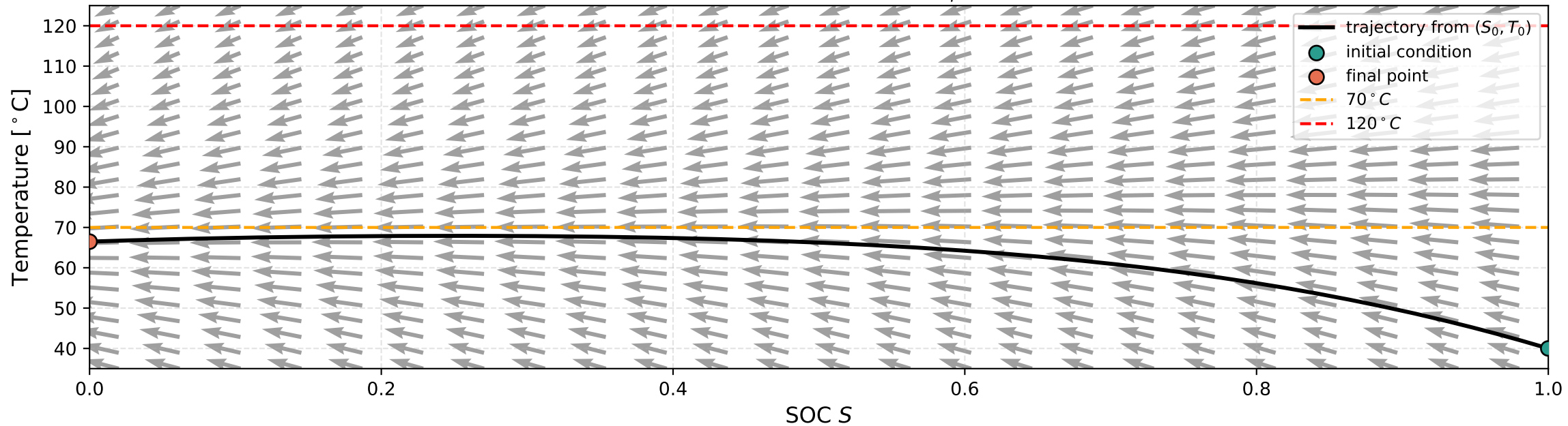
Vector field in the S - T plane, R_{isc} = 0.20\Omega , U_{eq} = 0.60 W/K, \varepsilon = 0.304
