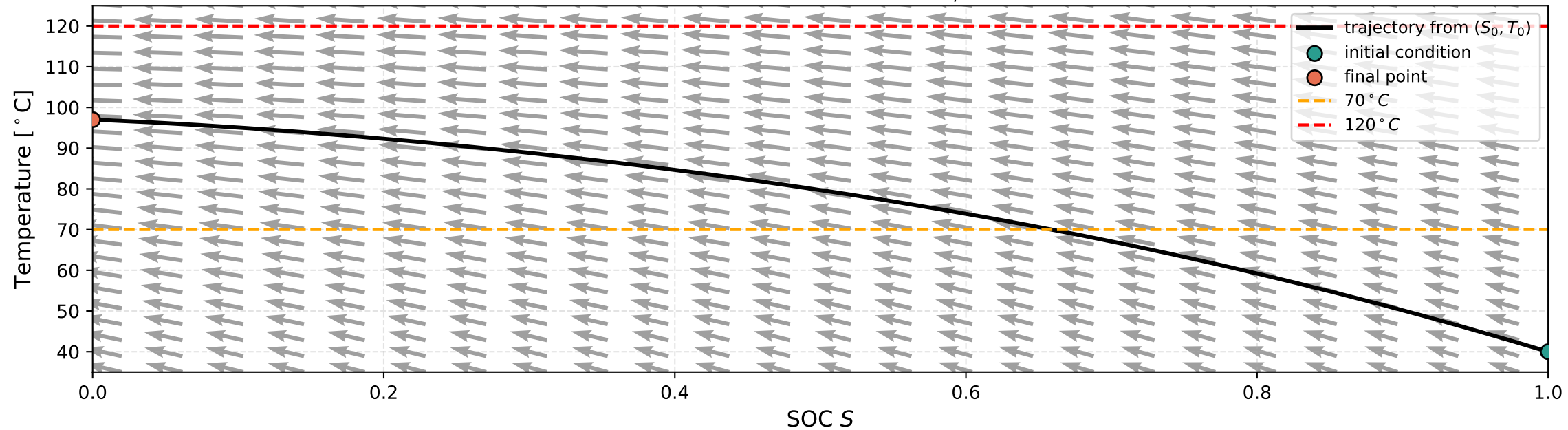
Vector field in the S - T plane, R_{isc} = 0.20\Omega , U_{eq} = 0.20 W/K, \varepsilon = 0.912
