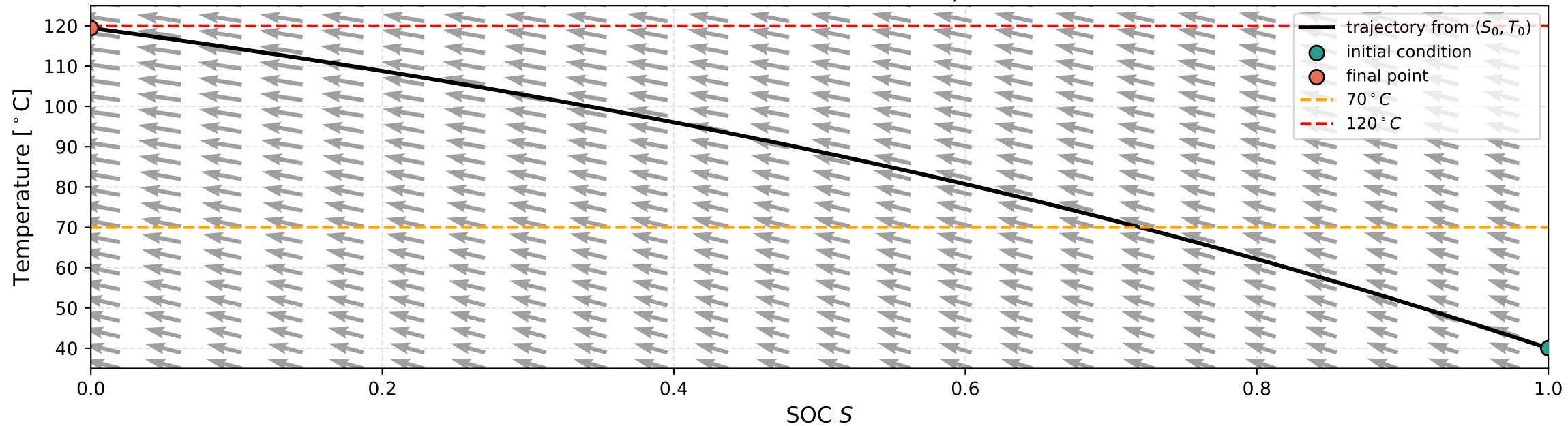
Vector field in the S - T plane, R_{isc} = 0.10\Omega , U_{eq} = 0.20 W/K, \varepsilon = 1.806
