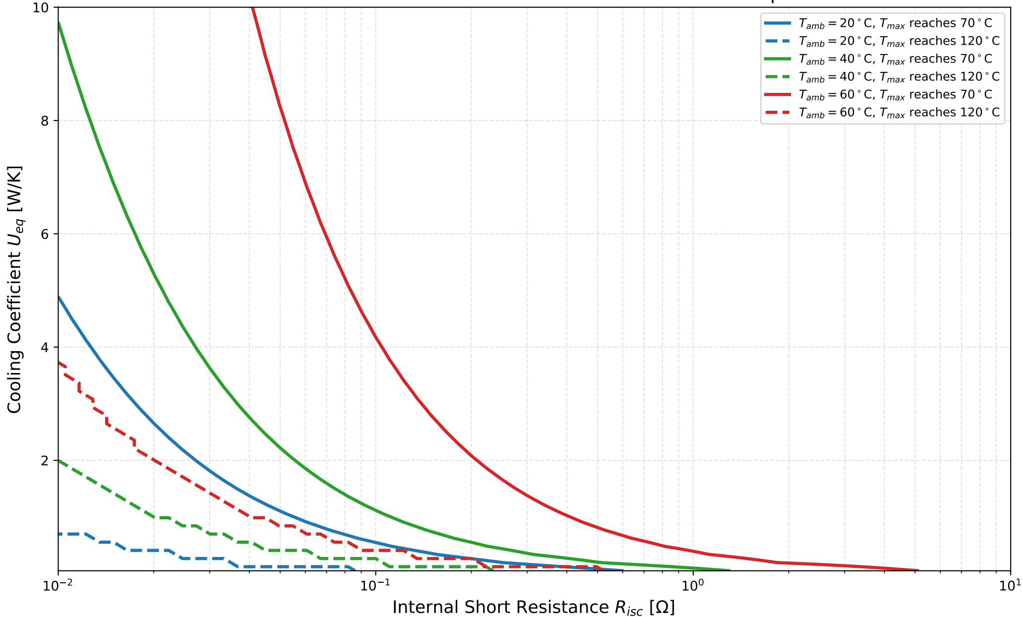
Simulated Thermal Boundaries under Different Ambient Temperatures
