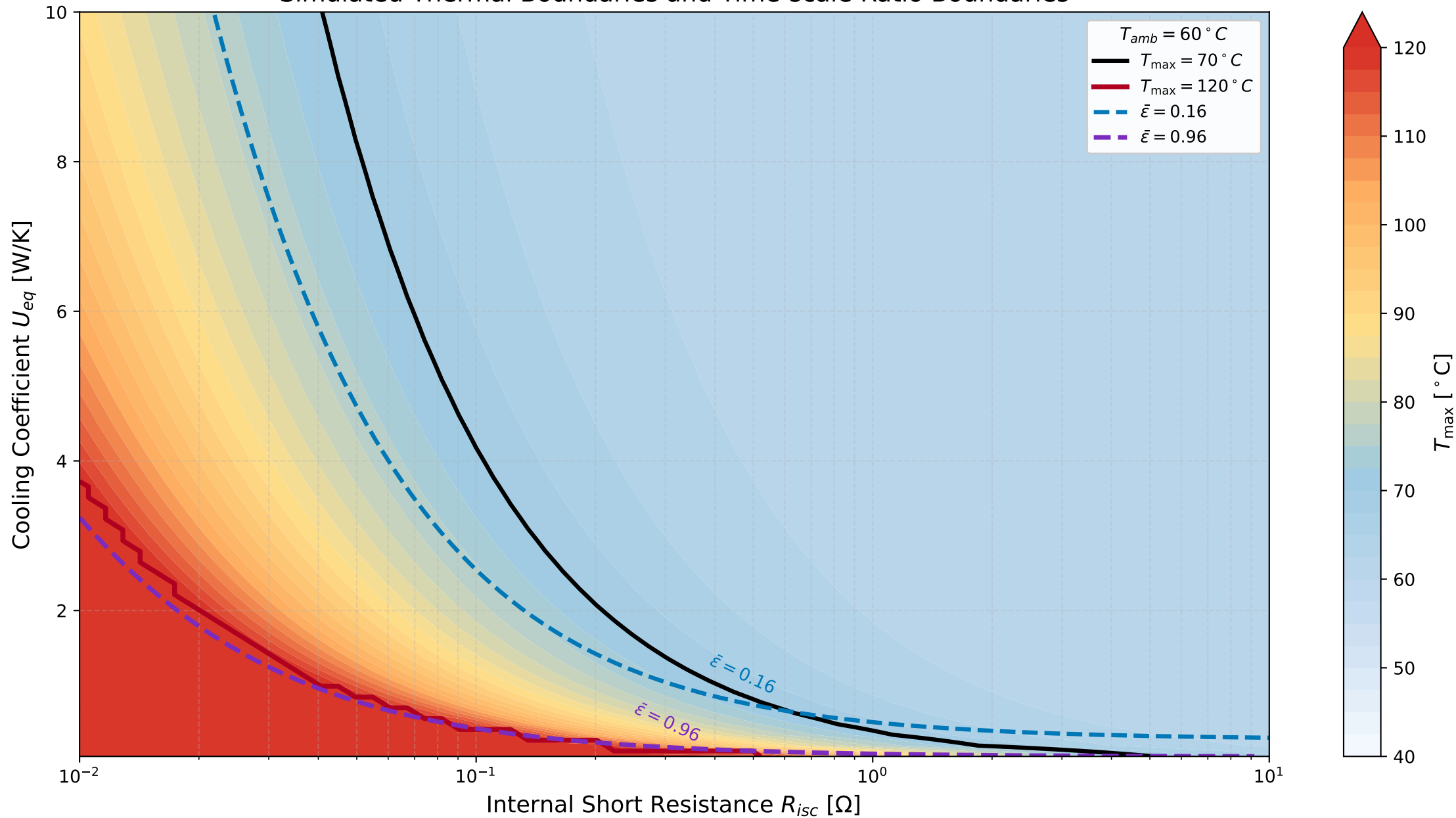
Simulated Thermal Boundaries and Time-scale Ratio Boundaries
