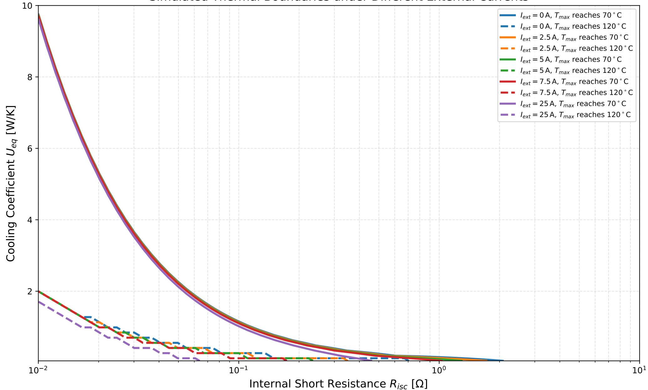
Simulated Thermal Boundaries under Different External Currents
