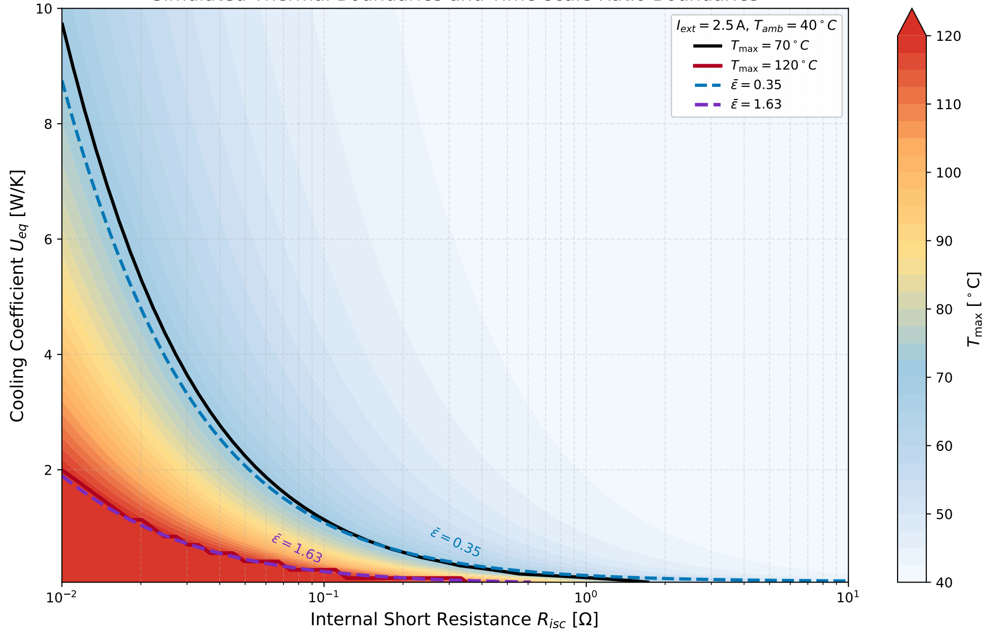
Simulated Thermal Boundaries and Time-scale Ratio Boundaries
