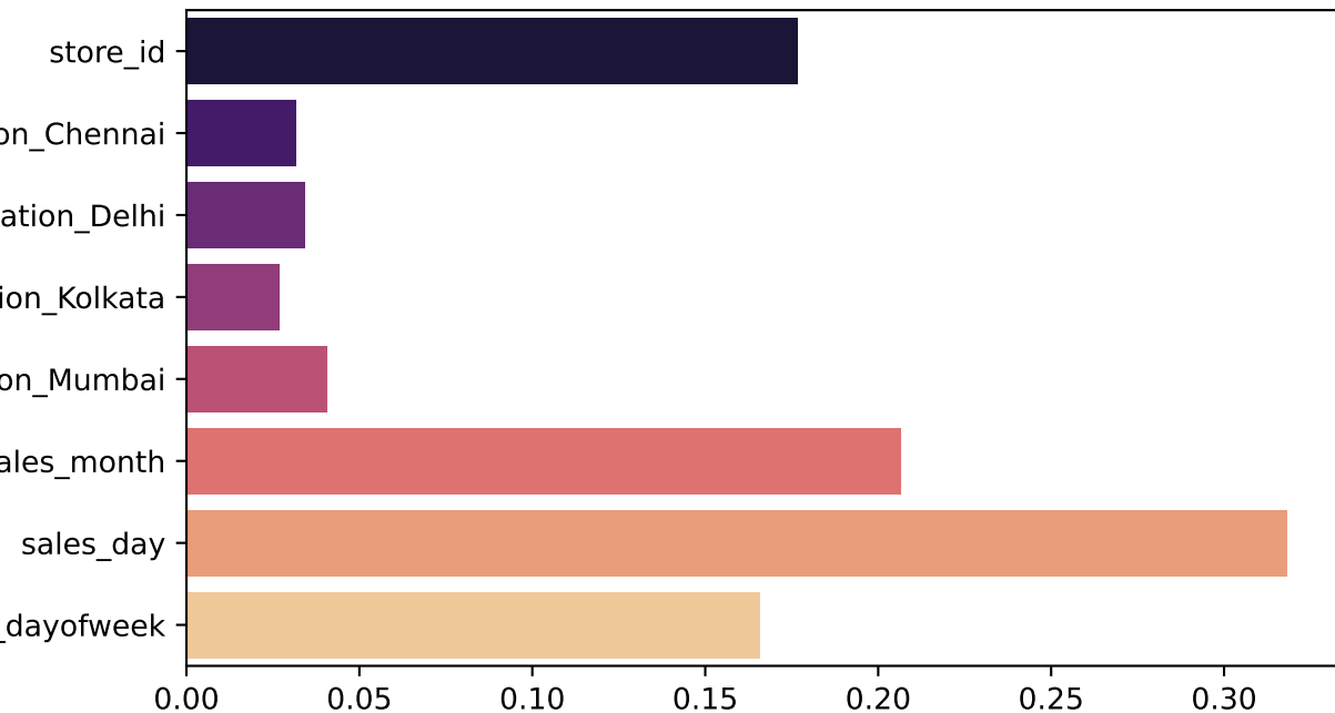
Task 3: Random Forest Feature Importance Rankings
