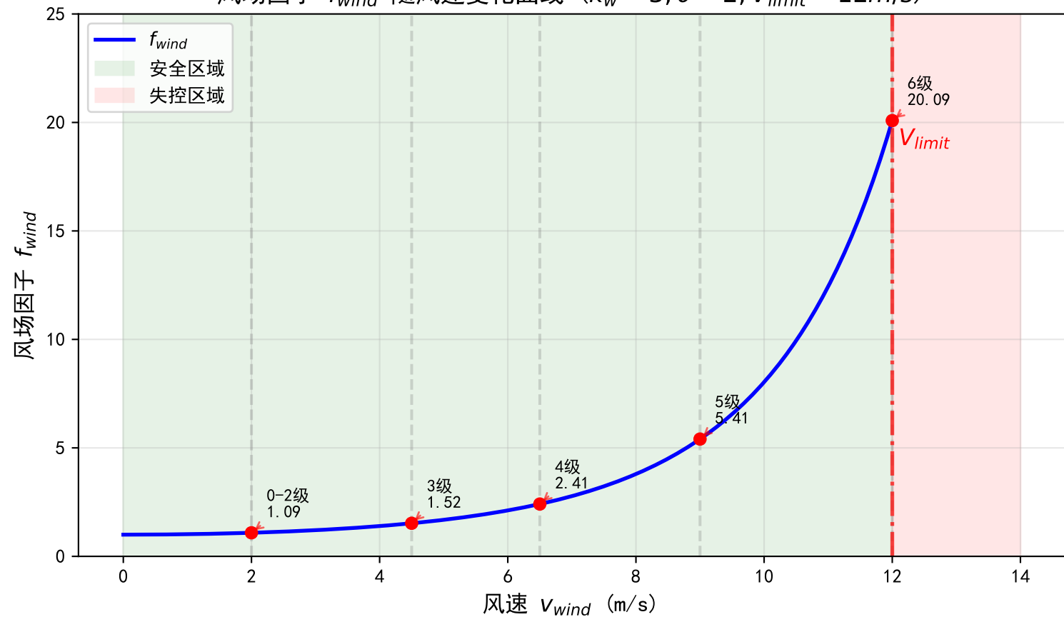
风场因子 f_{wind} 随风速变化曲线 ( k_w = 3, \theta = 2, V_{limit} = 12\text{m/s} )
