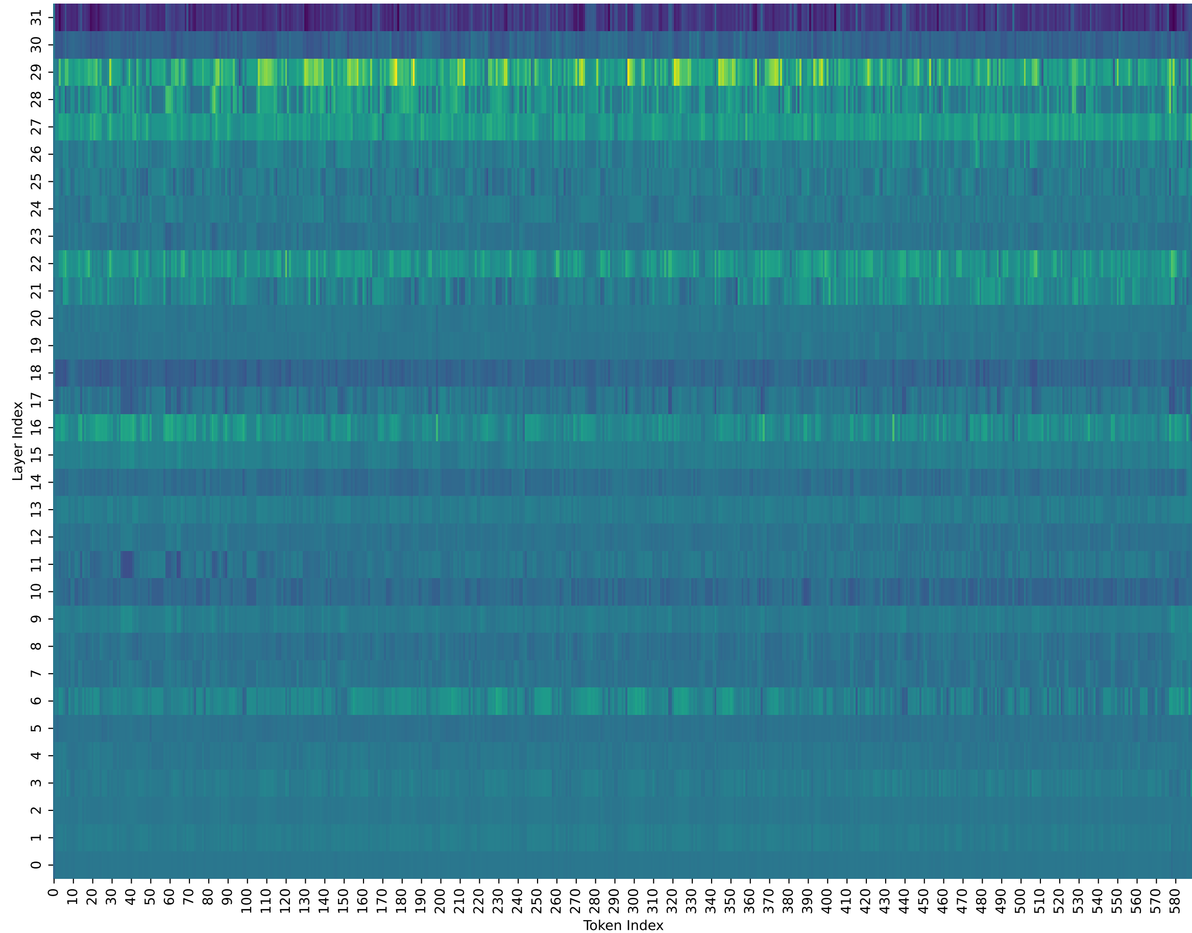
Activation Heatmap: Textual LoRA (Layers vs Tokens)
