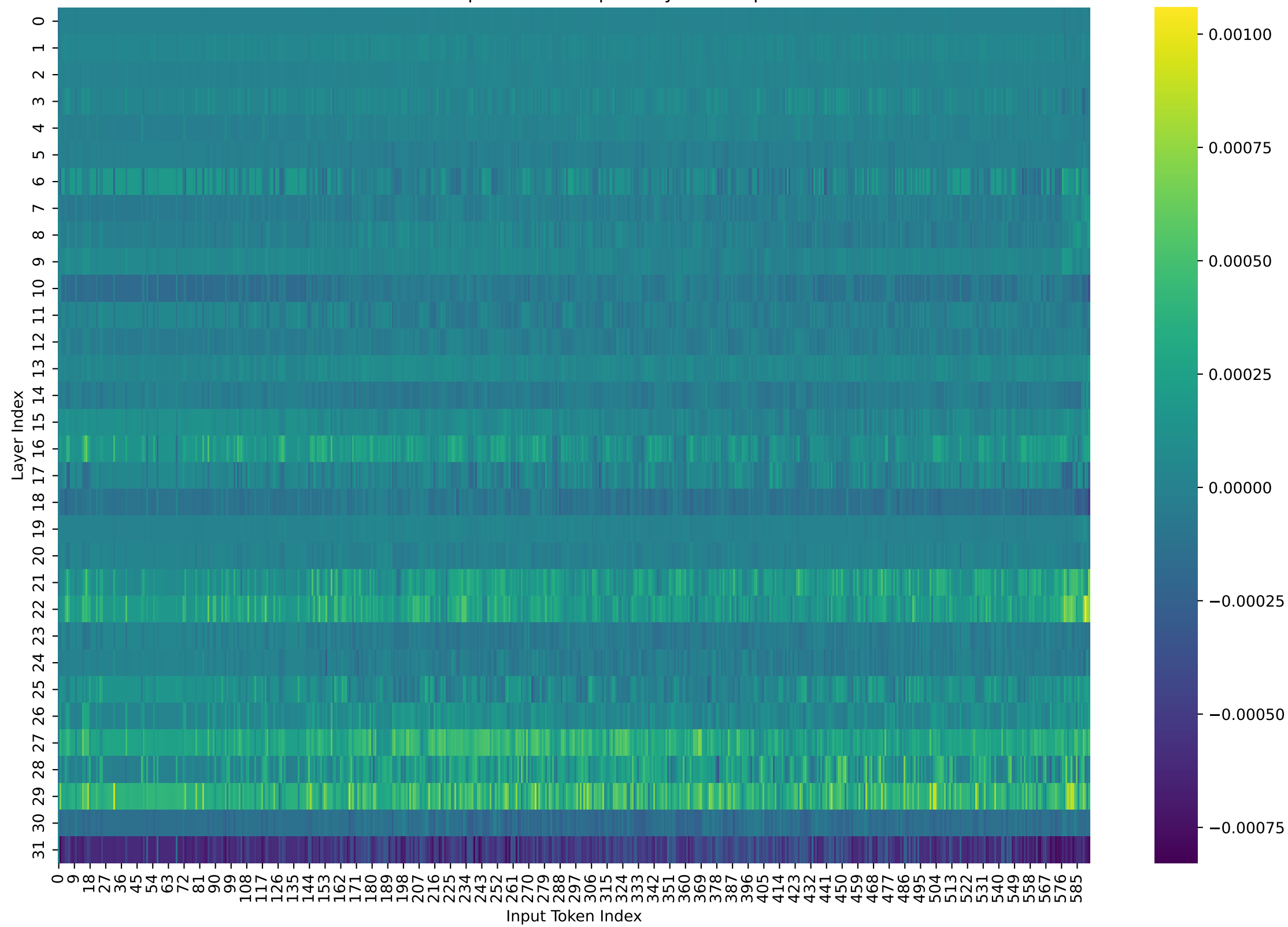
Activation Heatmap: Textual Adapter Layers vs Input Tokens
