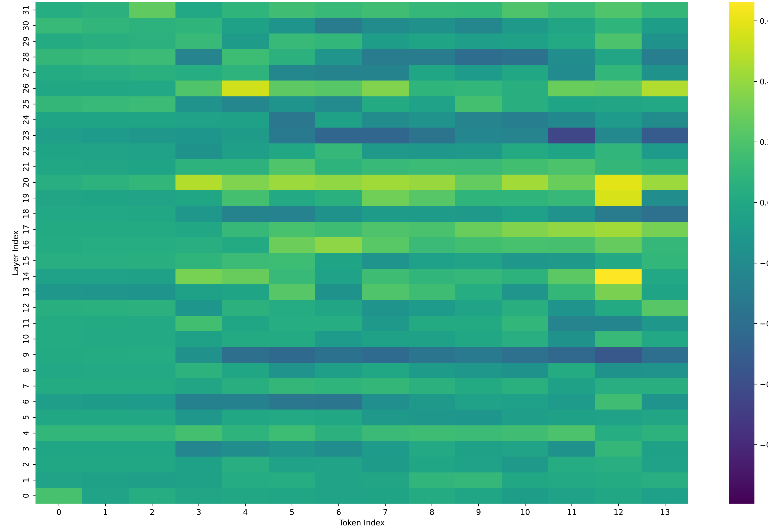
Activation Heatmap: Textual LoRA (Layers vs Tokens)
