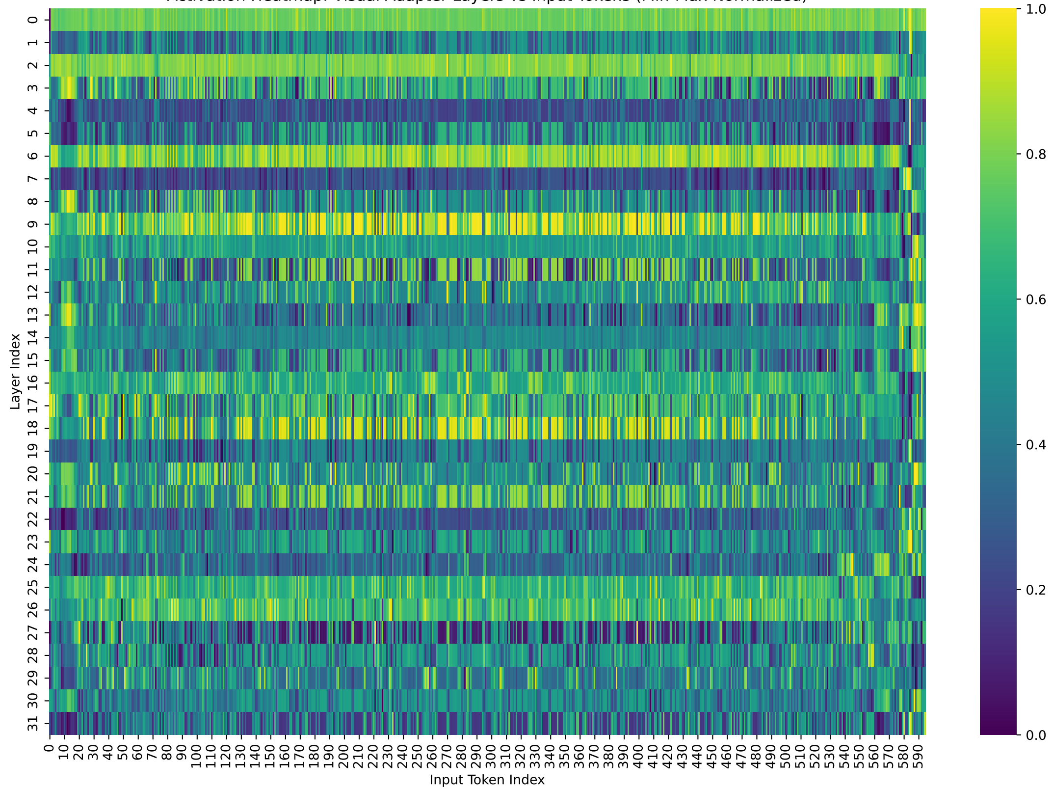
Activation Heatmap: Visual Adapter Layers vs Input Tokens (Min-Max Normalized)
