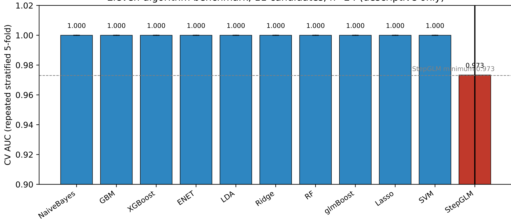
Eleven-algorithm benchmark, 11 candidates, n=24 (descriptive only)
