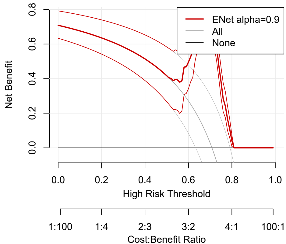
B Decision curve
