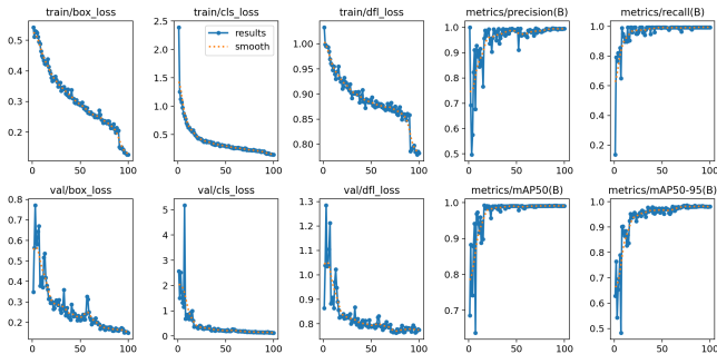
Fig. 3. Training losses and evaluation metrics over 100 epochs
