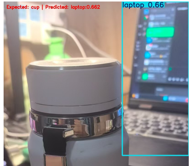
Fig. 7. Independent-test failure example: the true class is cup, but a background laptop is predicted as the target (04_cup.jpg)
