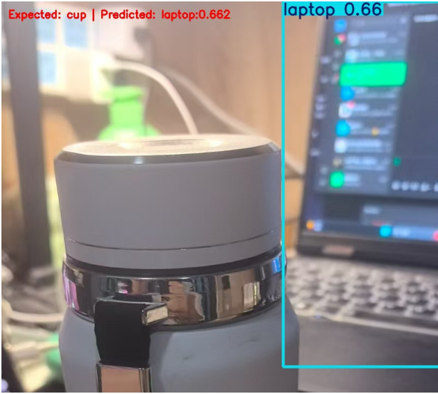
Fig. 7. Independent-test failure example: the true class is cup, but a background laptop is predicted as the target (04_cup.jpg)
