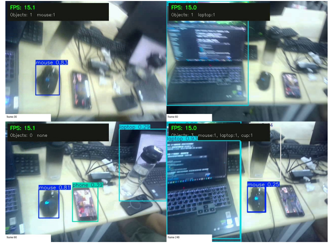
Fig. 6. Frames from the Jetson demonstration video, showing boxes, classes, confidence, object counts, and FPS
