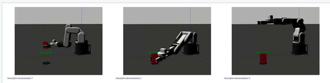
Simulation action sequence used for fixed-point pick-and-place verification
