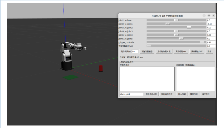
Manual teaching console and Gazebo scene used to establish the fixed points and verify the action sequence.
