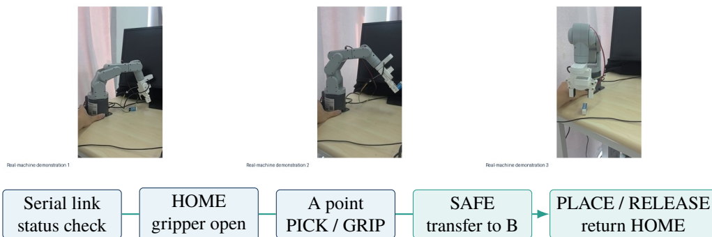
Figure 4. Real-machine frames paired with the action chain from device preparation to grasp, transfer, release and reset.
