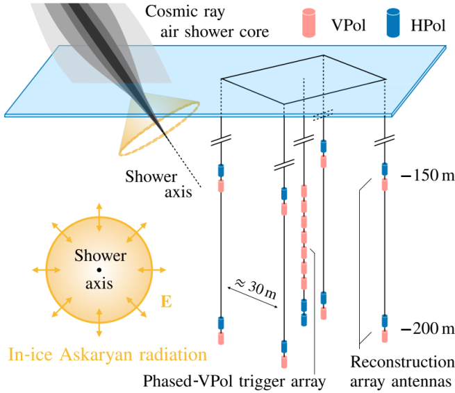
FIG. 2: The proposed UHECR candidate event geometry consists of a high-energy cascade interacting along the shower axis that enters the ice and creates Askaryan radiation. Figure adopted from [? ].
