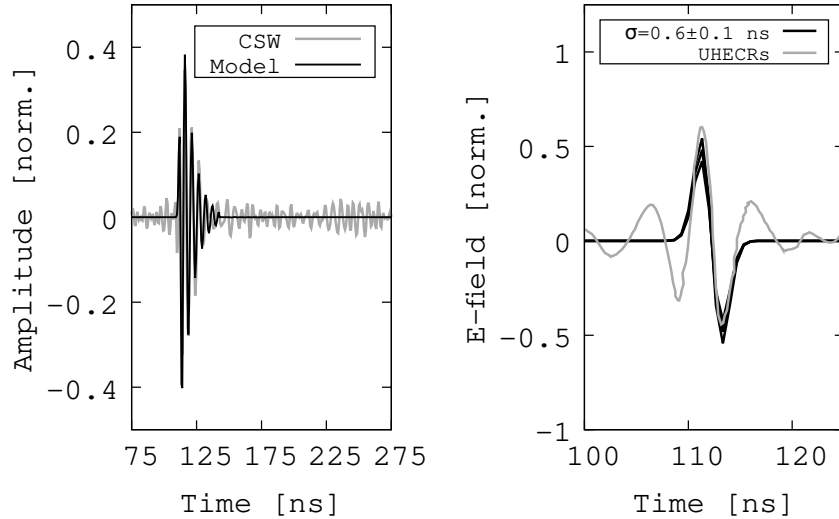
FIG. 7: (Left) The results from Fig. 4 bottom right, event ID 2716-58611. (Right) Equation 1, evaluated with the reconstructed \sigma_t from Tabs. II and III, and E_0 = 1 . Thick black line: \sigma_t = 0.6 ns. Thick gray lines: \sigma_t = 0.7 ns and \sigma_t = 0.5 ns. Thin black line: average data from UHECR \vec{E} -fields, adapted from Fig. 2 of [4].
