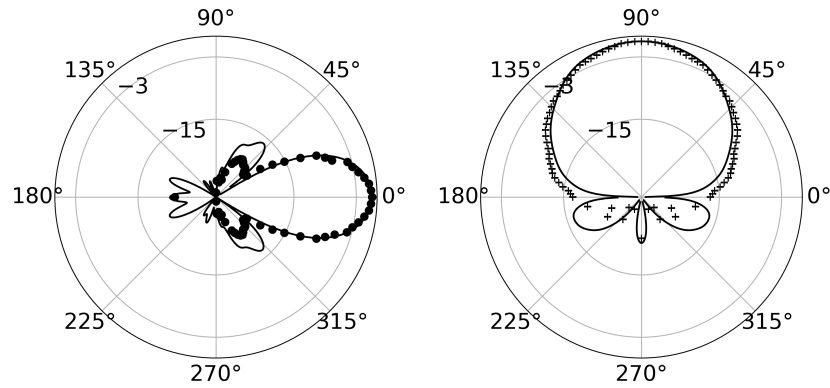
Figure 6. (Left) Black circles: the E-plane radiation pattern data ([5.8-6.0] GHz). Black line: 3D MEEP simulation of E-plane radiation pattern. (Right) Black crosses: the H-plane radiation pattern data ([5.8-6.0] GHz). Black line: 3D MEEP simulation of H-plane radiation pattern.
