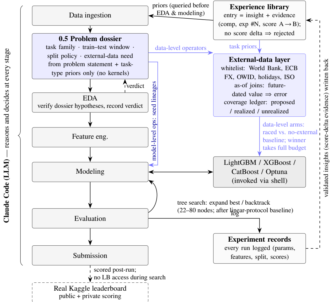
Figure 1: Architecture of my-agent. The LLM drives every stage; modeling and evaluation iterate via tree search, invoking Auto-ML tools through the shell, while the experience library and experiment records close the evidence loop. Blue: the injection layer (Section 2.2) — the Stage 0.5 dossier emits data-level operators that drive the external-data layer (whose arms race against the no-external baseline) and model-level operators that seed search lineages directly. The dossier is a prior, not a conclusion: EDA verifies its hypotheses and records a verdict. The leaderboard is external to the agent — lanes hold no credentials, and submissions are scored only after the run.
