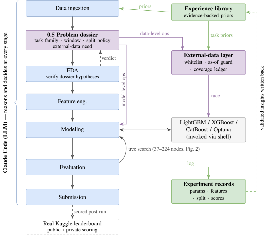
Figure 1: Architecture of the Sinica Kaggle Agent, with color marking role. Blue — the LLM-driven pipeline: Claude Code reasons and decides at every stage, and EDA records a verdict on the dossier’s hypotheses (the dossier is a prior, not a conclusion). Purple — the injection layer (Section 2.2): the Stage-0.5 dossier emits typed operators, data-level ones into the external-data layer’s arms, which race a no-external baseline with the winner taking the full budget, model-level ones directly into search lineages. Green — the evidence loop: the experience library and the experiment records, with validated insights written back. Gray — Auto-ML tools invoked via the shell. Dashed arrows mark feedback, advisory or post-run steps. The leaderboard is external to the agent: lanes hold no credentials, and submissions are scored only after the run.
