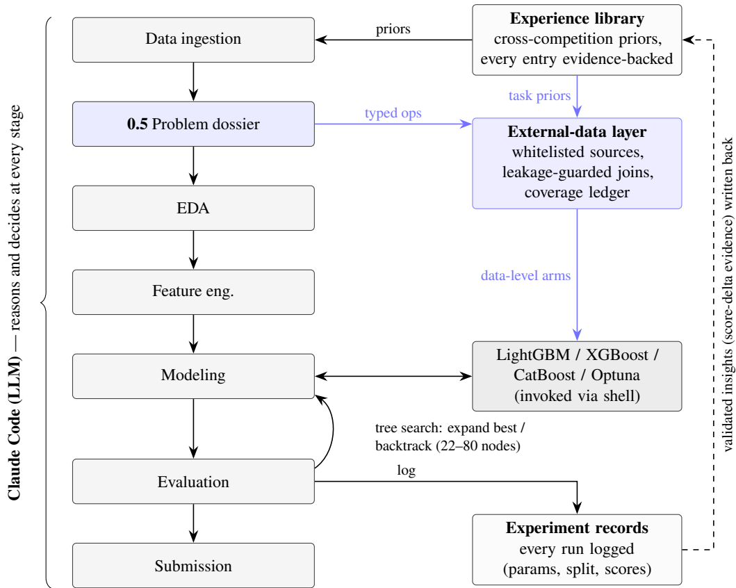
Figure 1: Architecture of my-agent. The LLM drives every stage; modeling and evaluation iterate via tree search, invoking Auto-ML tools through the shell, while the experience library and experiment records close the evidence loop. Blue: the injection layer (Section 2.2) — the Stage 0.5 dossier emits typed operators that drive the external-data layer, whose data-level arms race against the no-external baseline.
