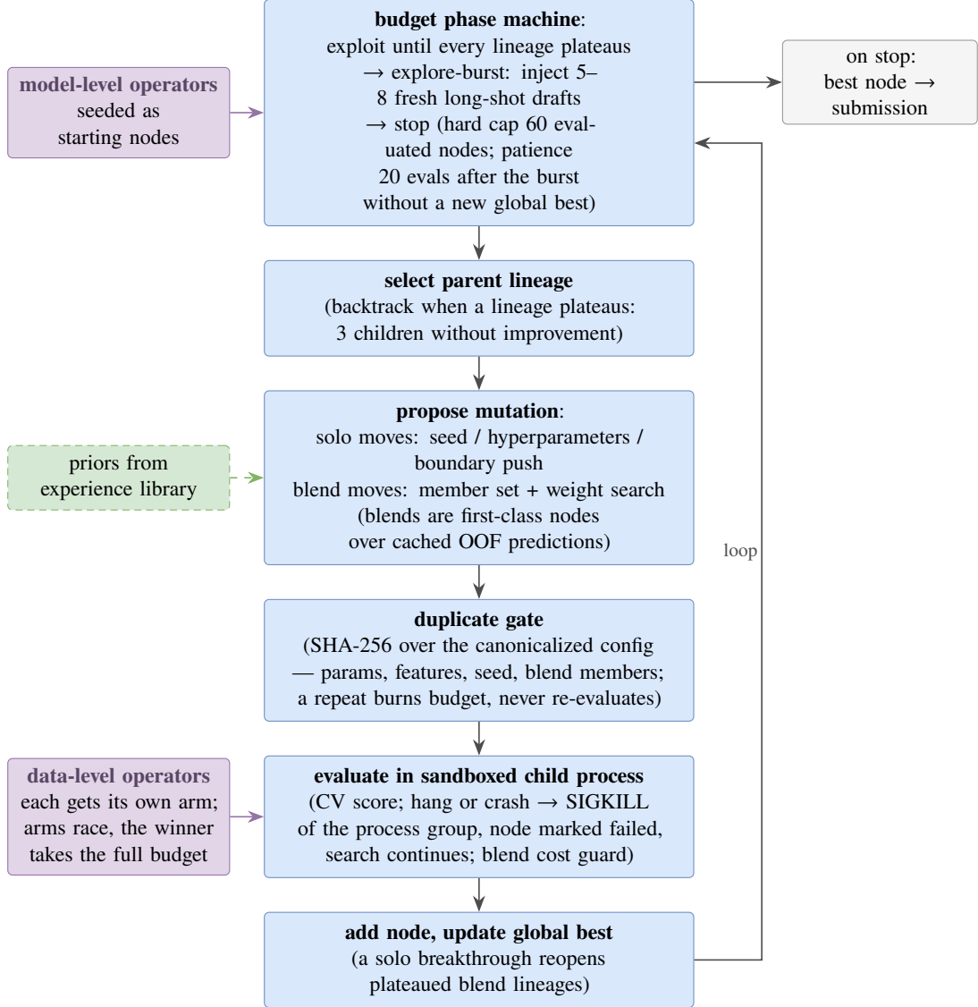
Figure 2: The tree-search loop used in all my-agent runs of this report (37–126 nodes per competition; per-competition counts in Table 11). Each node is a complete, executable solution scored by local cross-validation; lineages are abandoned on plateau, and the budget phase machine forces one exploration burst before stopping. Figure 3 shows what the loop builds. Purple: the injection layer’s operator entry points (Section 2.2) — model-level operators seed starting nodes; data-level operators build separately raced arms. Green: priors from the experience library. Solid arrows: the loop’s execution flow; dashed: advisory input and backtracking.
