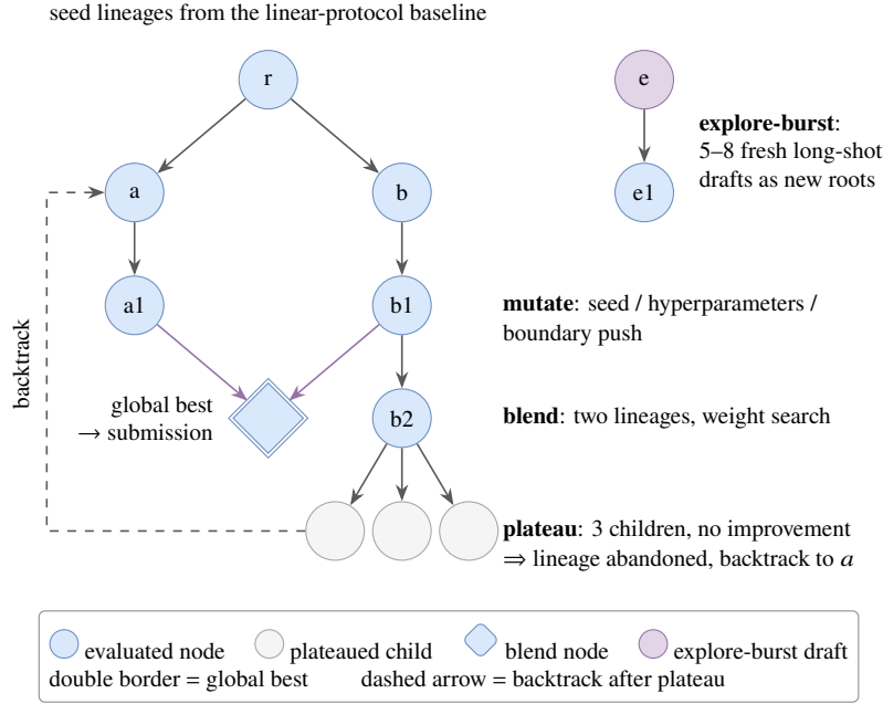
Figure 3: What the loop of Figure 2 builds: one search tree, schematic. Two lineages grow from the linear-protocol baseline; lineage b plateaus after three children fail to improve, so the search backtracks and abandons it; a blend node over the cached out-of-fold predictions of a1 and b1 becomes the global best and is what gets submitted; the forced explore-burst injects fresh long-shot drafts ( e ) as new roots. Node labels are schematic — real runs evaluate 37–126 nodes per competition (Table 11).
