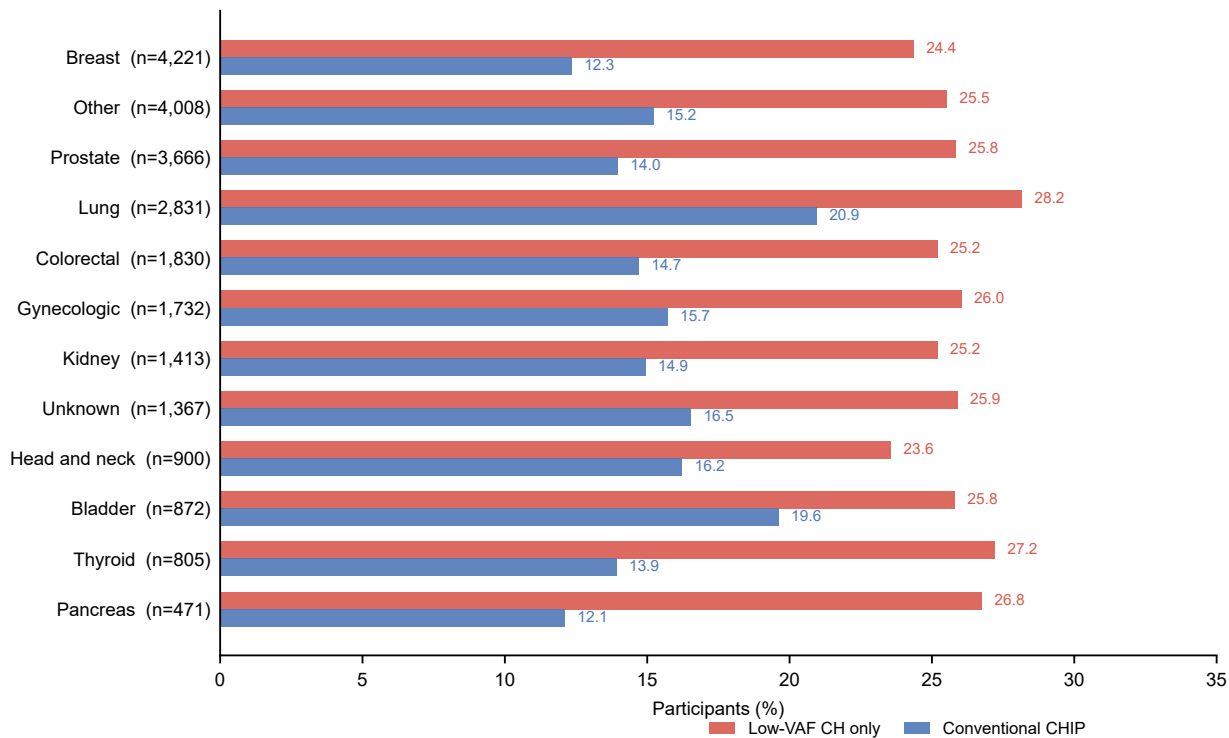
Observed CH prevalence across solid-tumor groups
